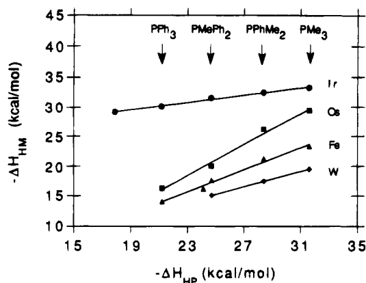
Figure 2. Correlations of metal basicity ( -\Delta H_{\text{HM}} ) with phosphine basicity ( -\Delta H_{\text{HP}} ) for \text{CpIr}(\text{CO})(\text{PR}_3) , \text{CpOs}(\text{PR}_3)_2\text{Br} , \text{Fe}(\text{CO})_3(\text{PR}_3)_2 , and fac - \text{W}(\text{CO})_3(\text{PR}_3)_3 (eqs 13–20).
